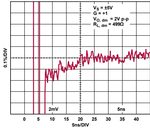
Figure 44. 0.1% Settling Time
